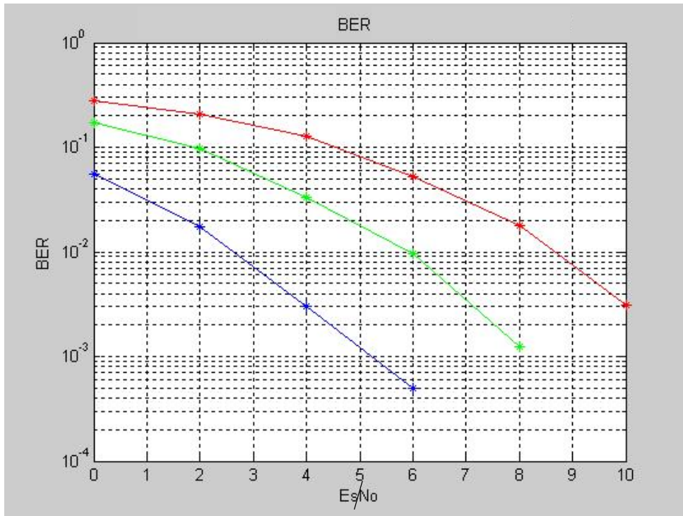
Figure 4: BER for AWGN channel, spreading frequency 11MHz versus Es/No for different data rates: red – 1MB/s, green – 0,5 Mb/s, blue- 0,25 Mb/s
