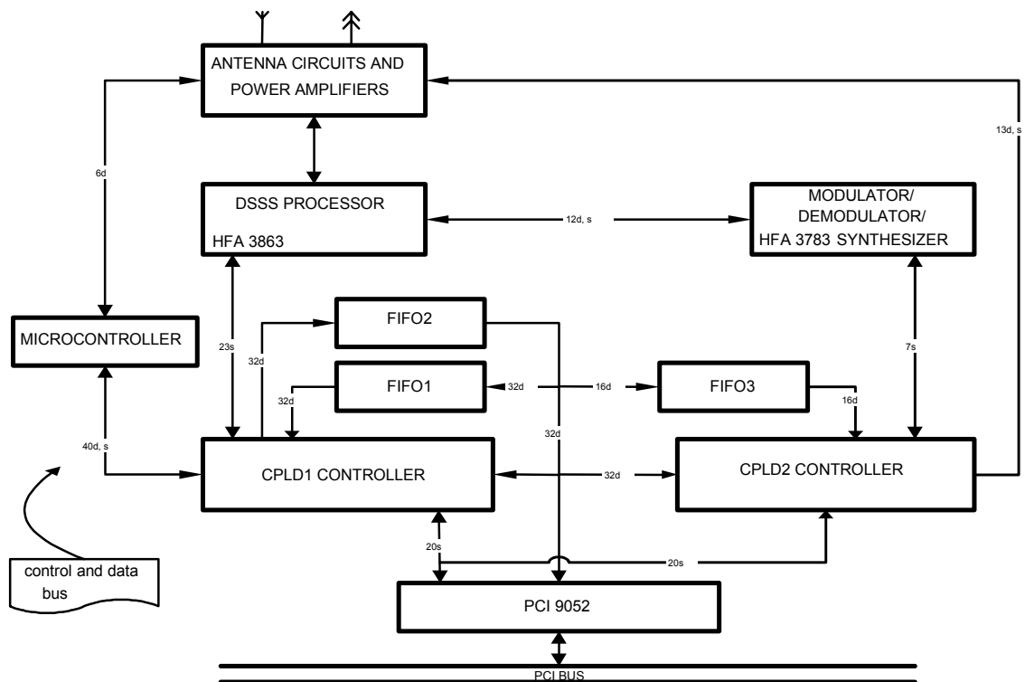
Figure 1: Block diagram of designed MILWLAN board
