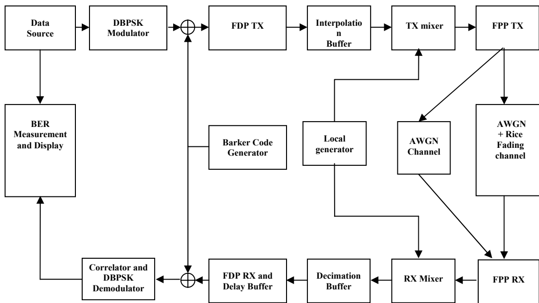
Figure 3: Block diagram of simulation model
