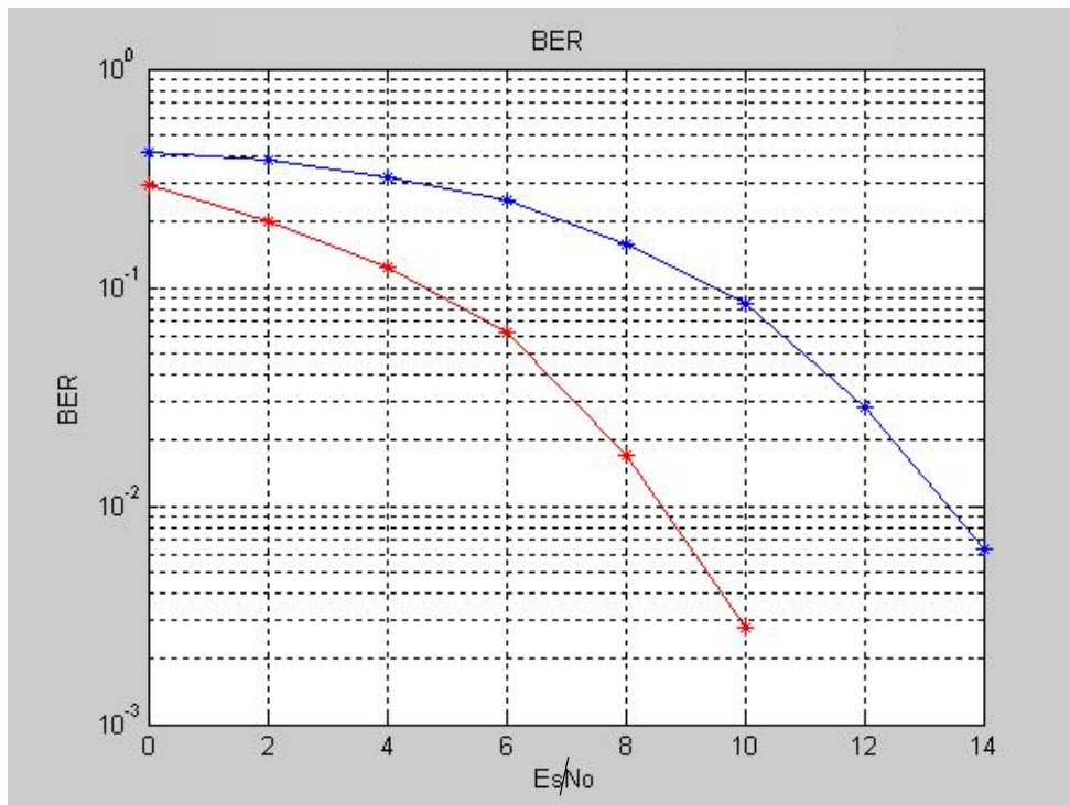
Figure 5: BER for AWGN channel and 6 path Rician fading, spreading frequency 11MHz and data rate – 1MB/s versus Es/No: red – AWGN channel, blue- AWGN channel plus Rician fading
